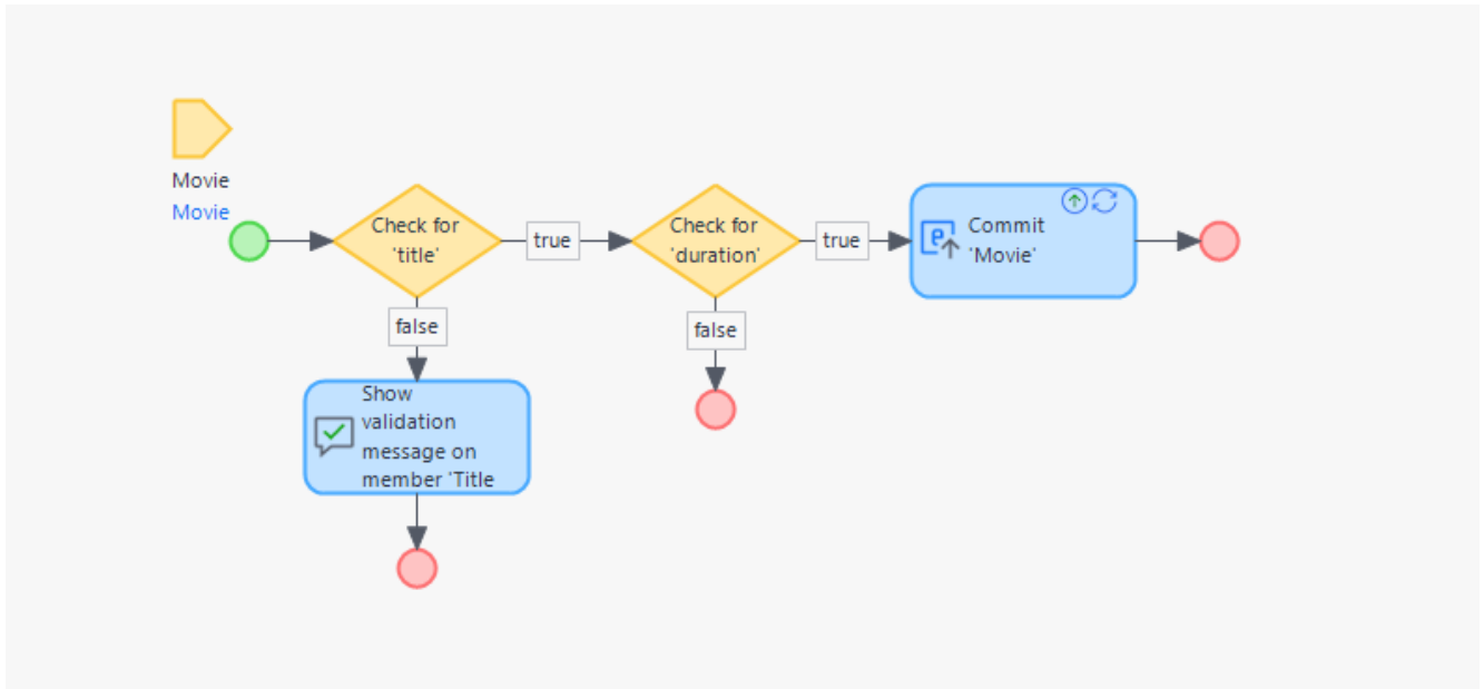
Figure 2. Microflow: ACT_Movie_Save
