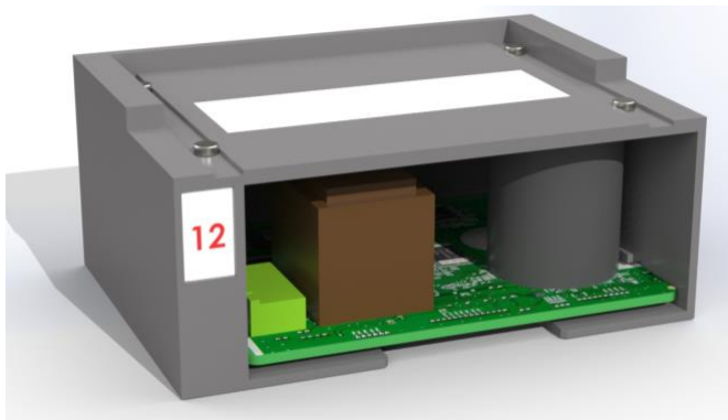
Figure 6. Protective housing for custom PCBA (design renderings).
