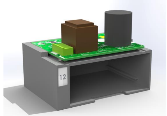
Figure 6. Protective housing for custom PCBA (design renderings).
