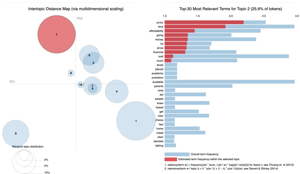
Figure 3: Topic modeling using LDA representing topic 2 most salient words.
