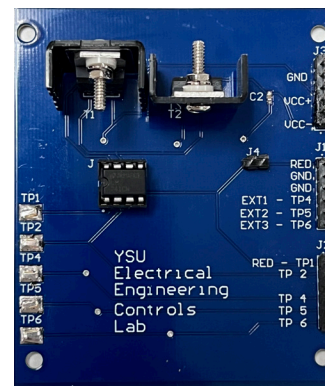
Figure 12b: PCB
