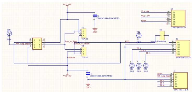
Figure 12a: Altium Designer Schematic for the PCB.
