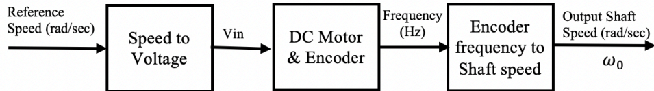
Figure 4a: DC motor open-loop system
